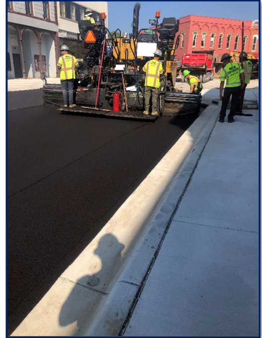
Fig 1: Michigan Paving paves the base course of asphalt along Brady St
