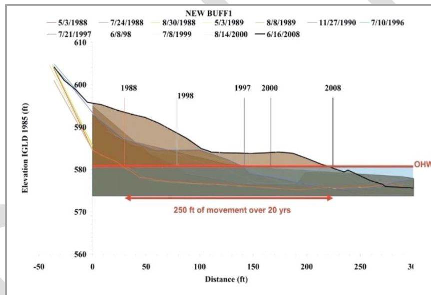
Figure 7. Beach profile showing movement of the elevation ordinary high-water mark (E-OHWM) through time (from Meadows, 2021).
