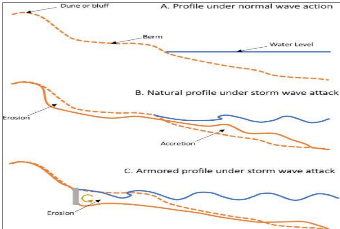
Figure 3. Profile response for natural and armored beaches (Meadows, Xue, Ye, Huang, & Kayastha, 2021)
