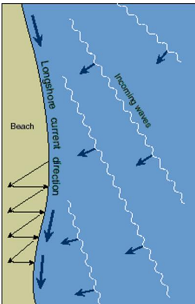
Figure 4. Longshore drift process. Source: USGS
