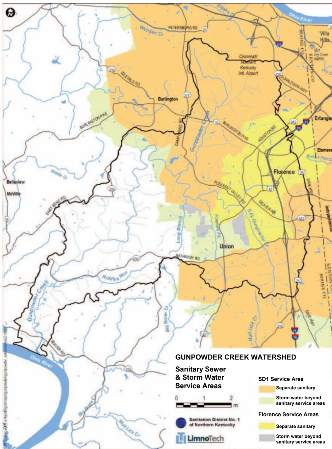
Figure 5-8: Sanitary sewer &amp; stormwater service areas within the Gunpowder Creek Watershed (LTI, 2009)
