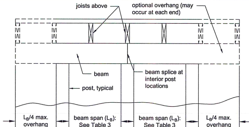
Figure 3. Beam Span.
