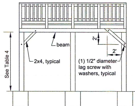
Figure 10. Diagonal Bracing.
