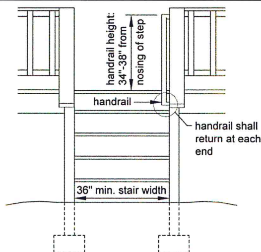
Figure 33. Miscellaneous Stair Requirements.
