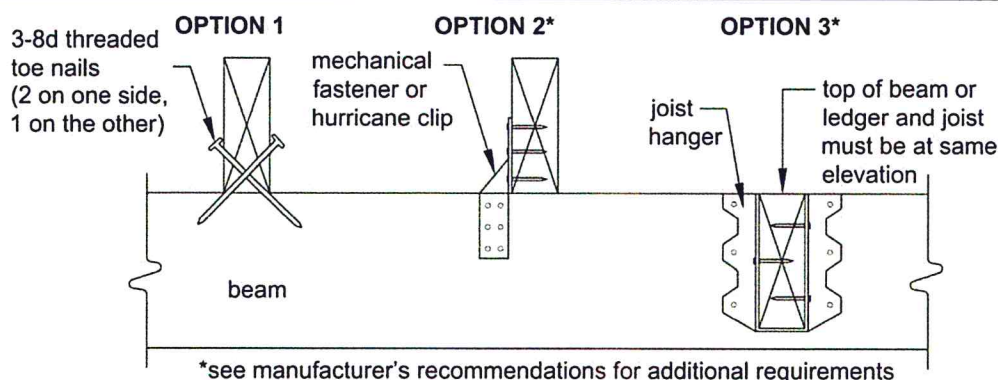
Figure 6. Joist-to-Beam Detail.
