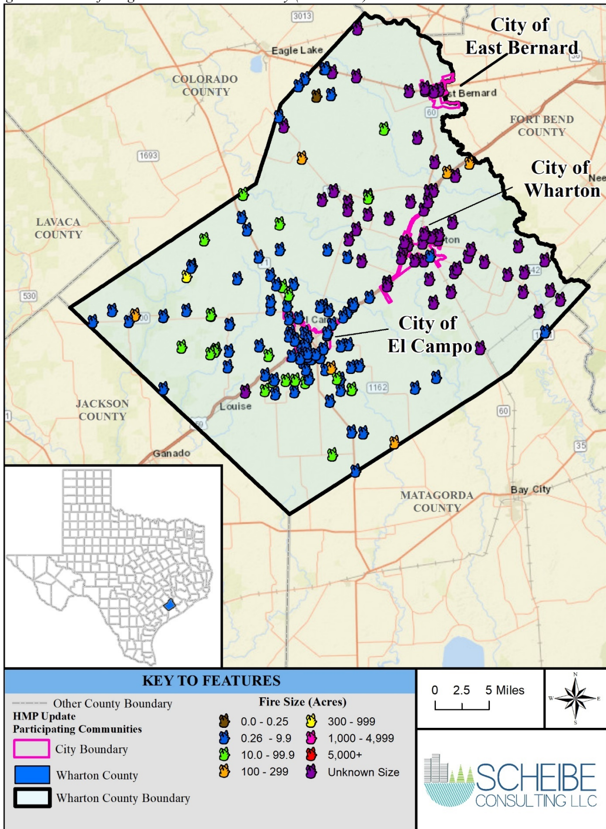
Figure 16-2. Wildfire Ignitions in Wharton County (2005-2021)
