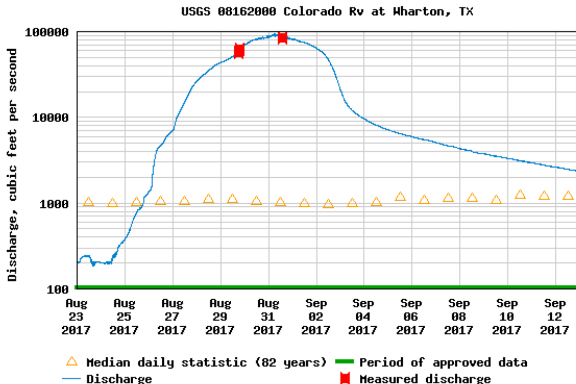
Figure 12-3. Colorado River Flow Near the City of Wharton During Hurricane Harvey
