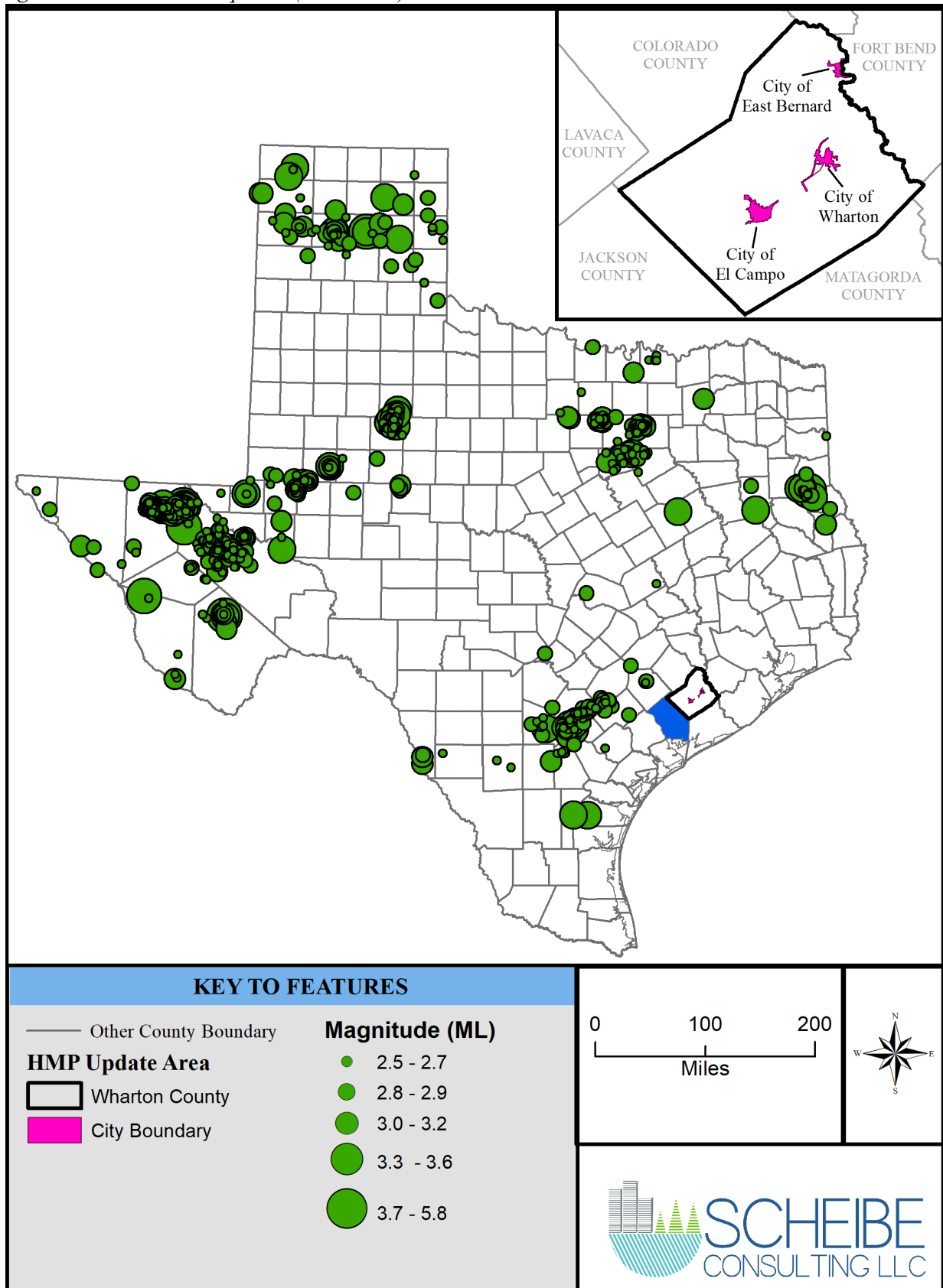
Figure 11-1. Texas Earthquakes (1847-2021)
