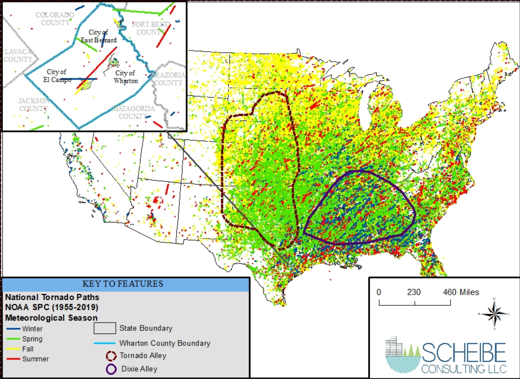
Figure 15-3. Tornado Paths in the U.S. (1955-2019)
