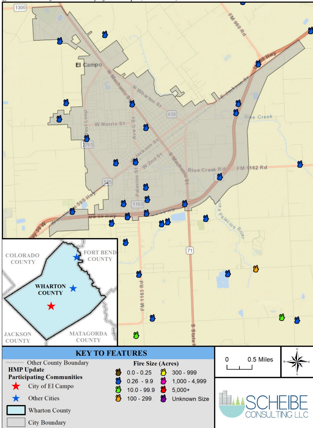
Figure 16-4. Wildfires in the City of El Campo (2005-2021)
