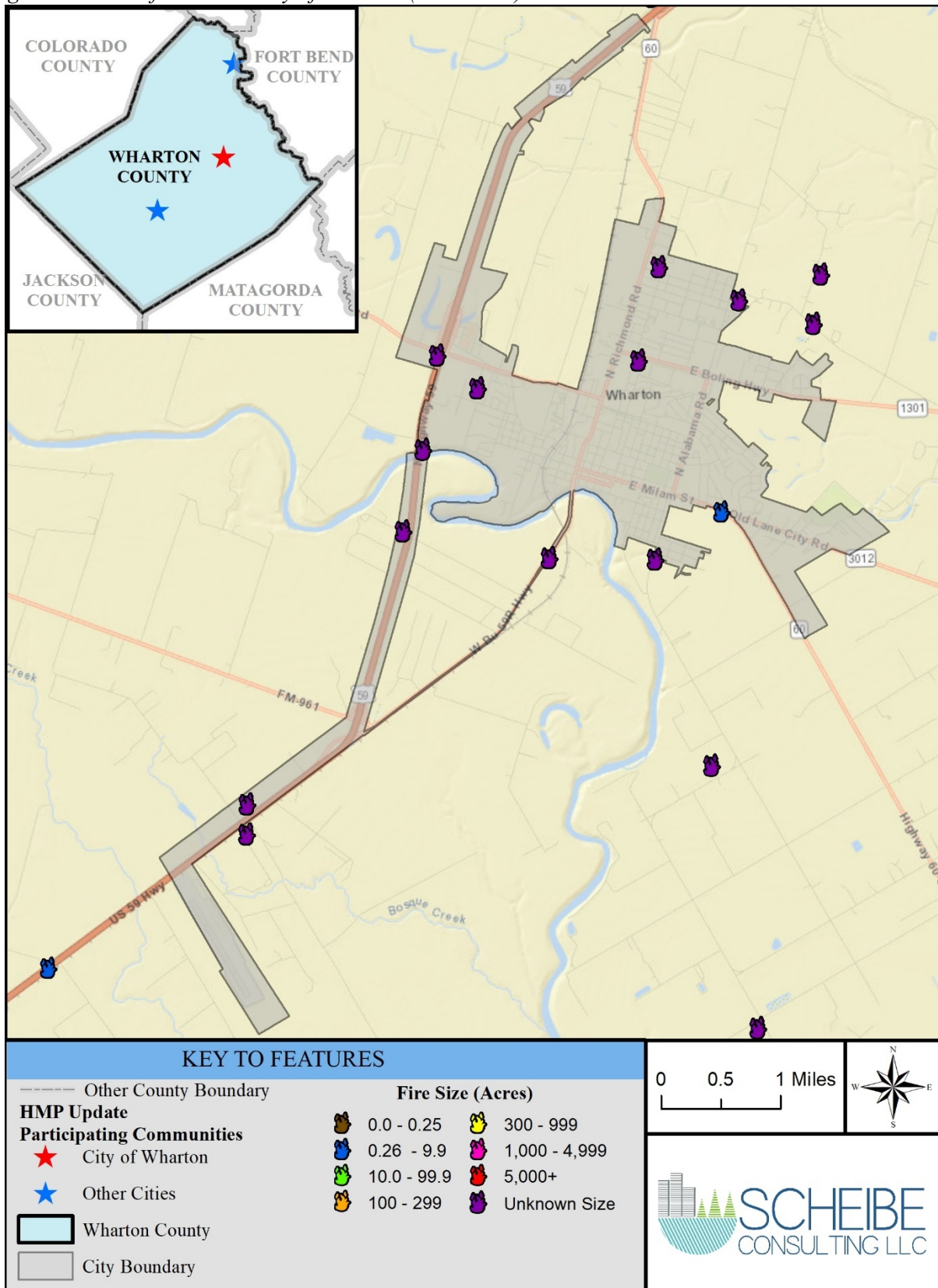
Figure 16-5. Wildfires in the City of Wharton (2005-2021)
