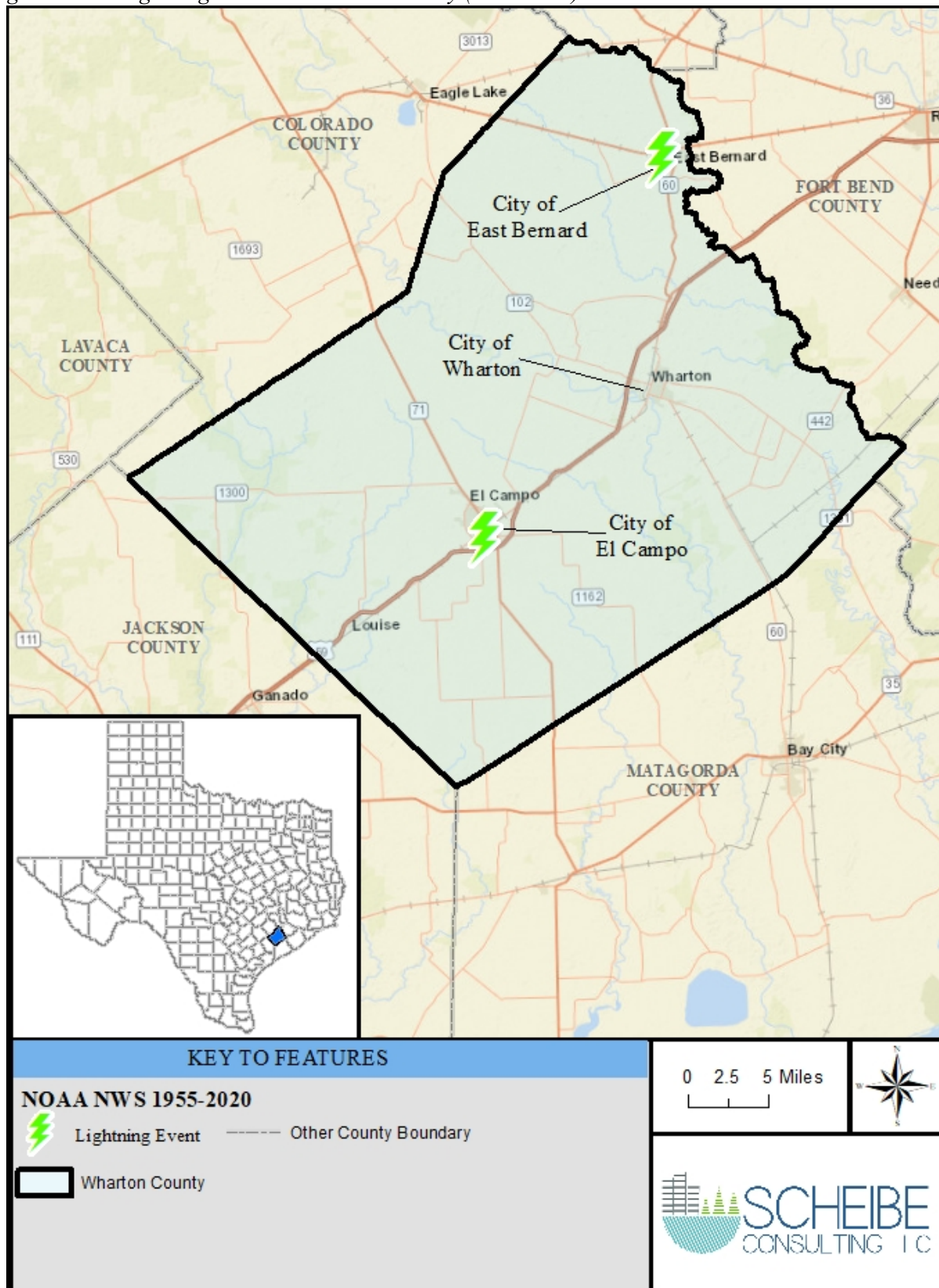
Figure 14-10. Lightning Events in Wharton County (1955-2020)
