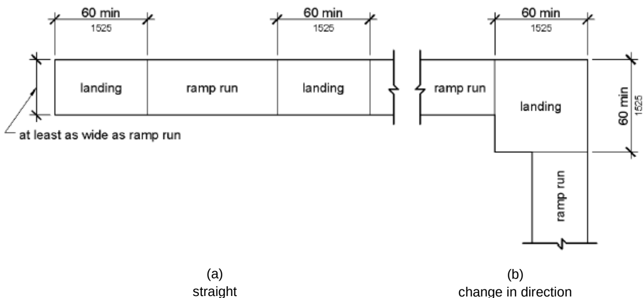
Figure 405.7 Ramp Landings
