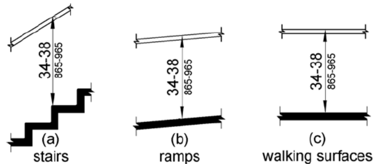
Figure 505.4 Handrail Height
