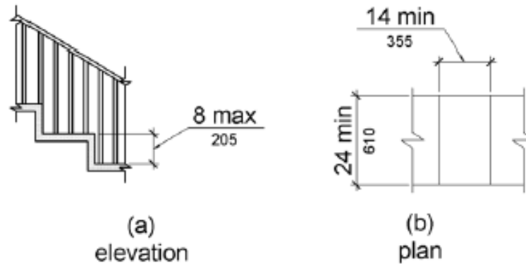
Figure 1008.3.2 Transfer Steps
