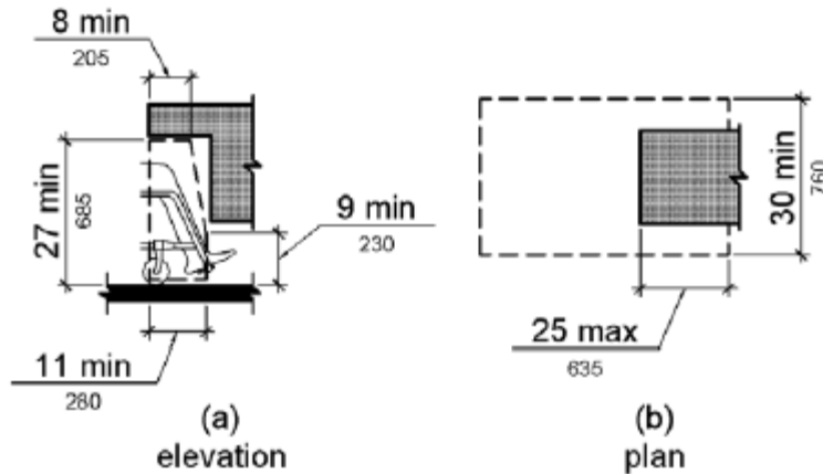
Figure 306.3 Knee Clearance
