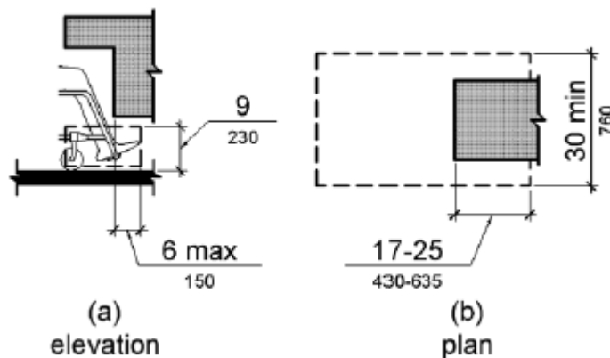
Figure 306.2 Toe Clearance
