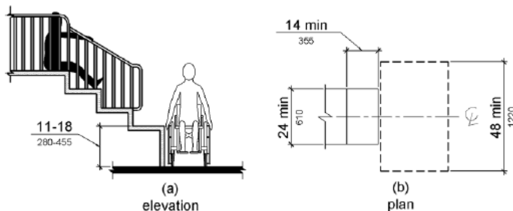
Figure 1008.3.1 Transfer Platforms
