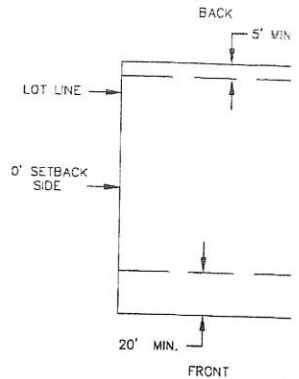
TYPICAL SETBACKS D: FOR TRACTS A-5-1 THRU A-5-5 (N.T.S.)
