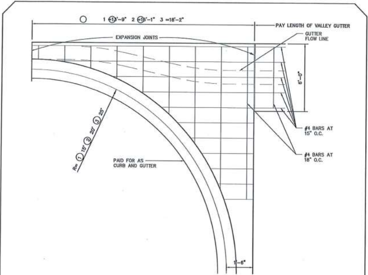
VALLEY GUTTER DETAIL
