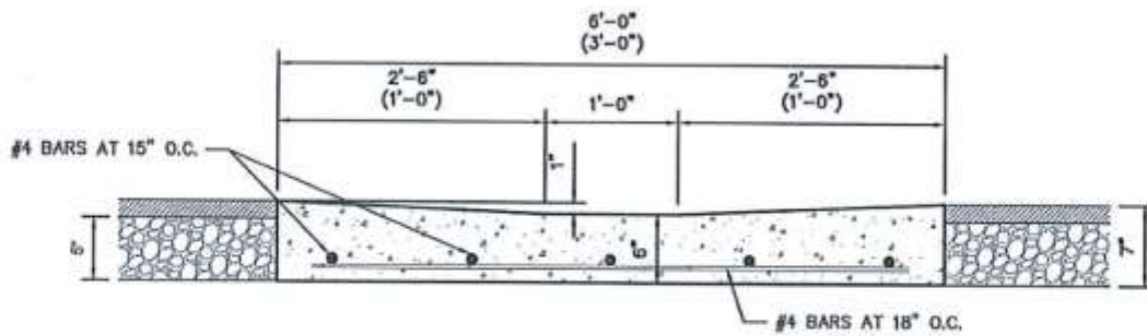
TYPICAL VALLEY GUTTER SECTION
