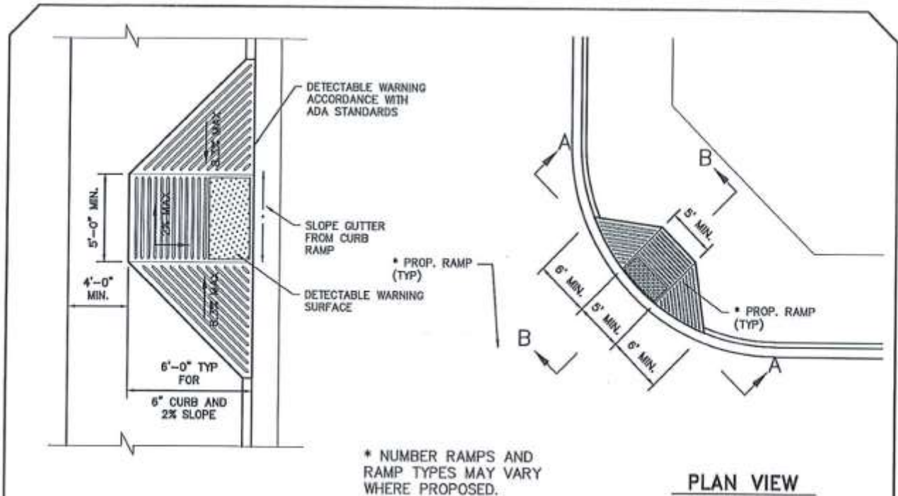
PLAN VIEW
