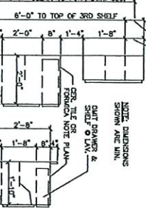
SECTION THRU BATH & KITCHEN CABINETS
