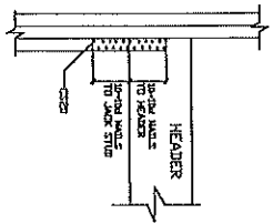
DETAIL 7A
