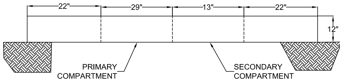
SIDE VIEW
