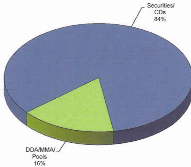
Portfolio Composition
