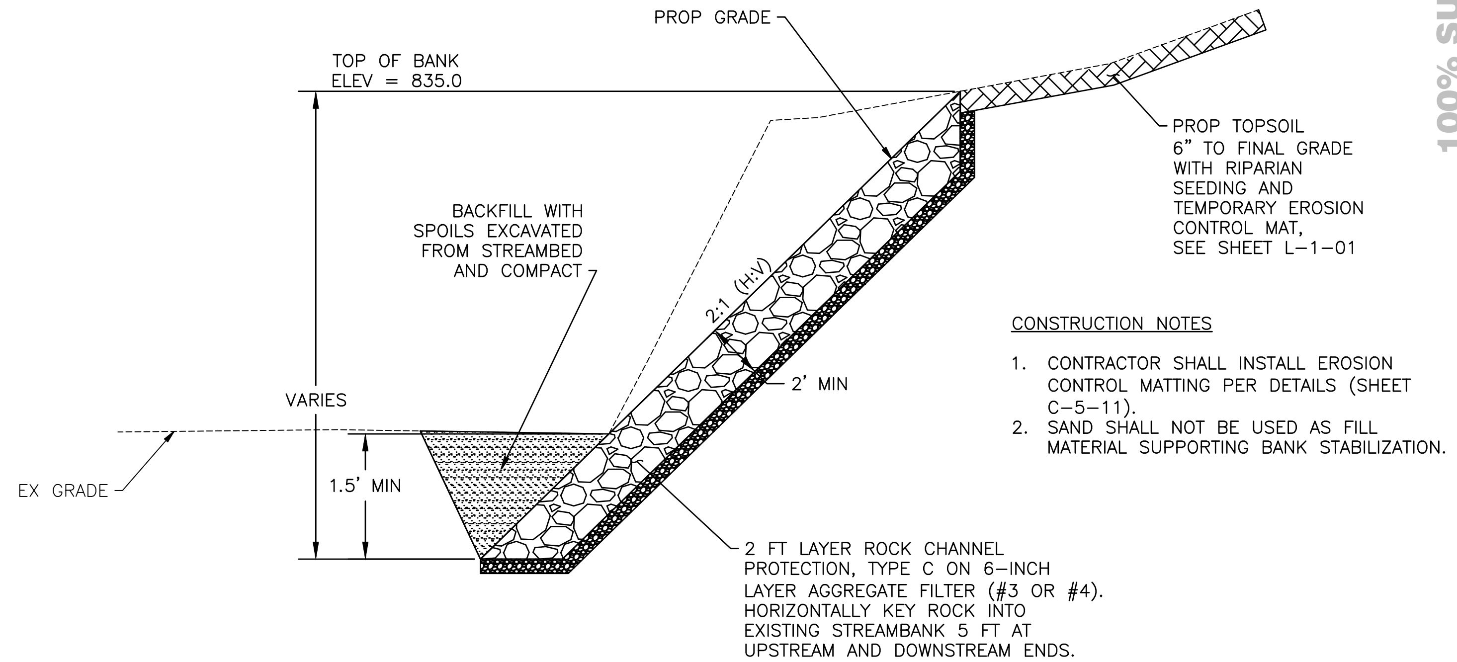
DETAIL BANK STABILIZATION - STA 4+58 TO 5+07, RIGHT (NORTH BANK) NOT TO SCALE
