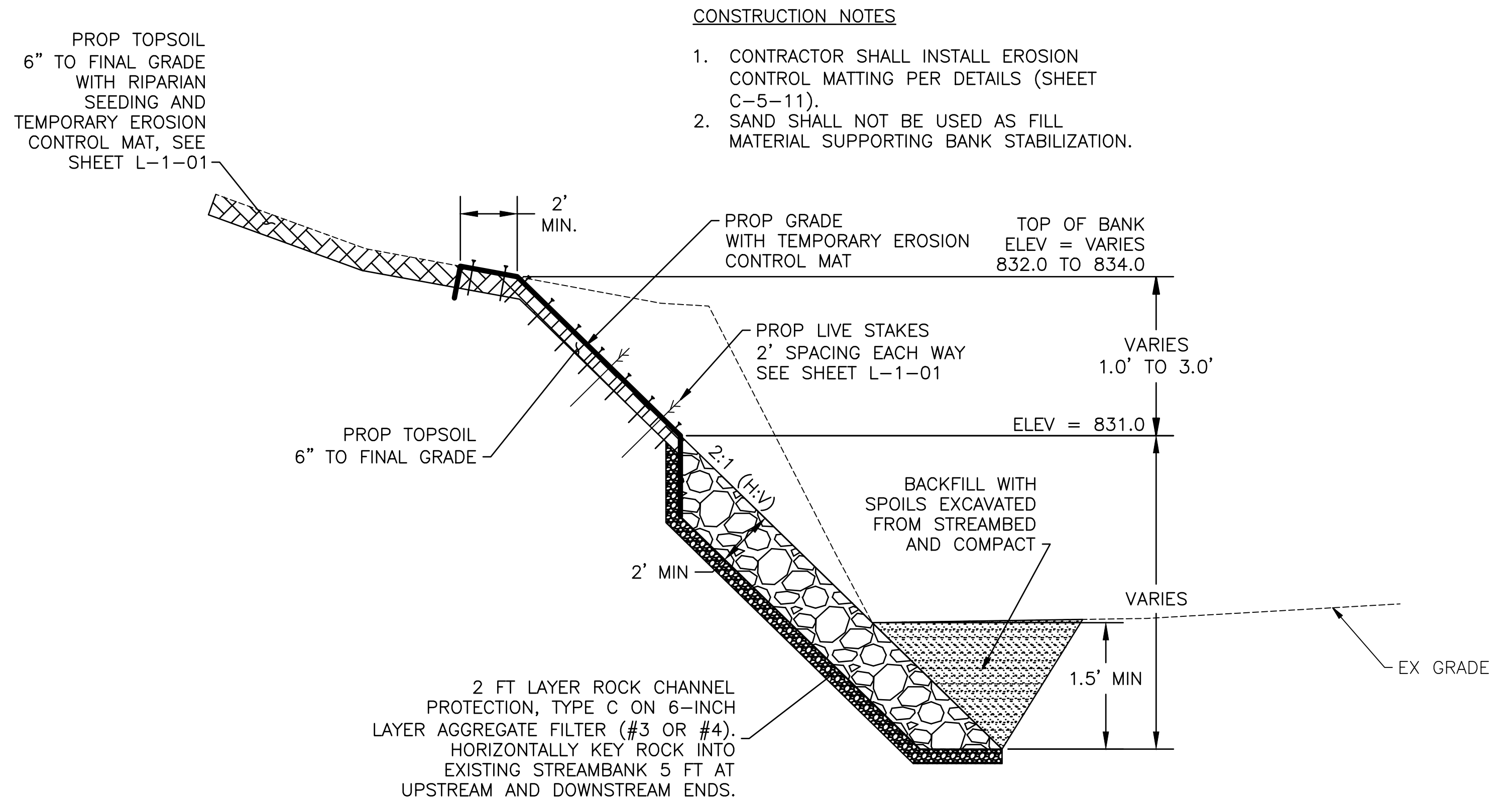
DETAIL BANK STABILIZATION - STA 4+97 TO 5+80, LEFT (SOUTH BANK) NOT TO SCALE
