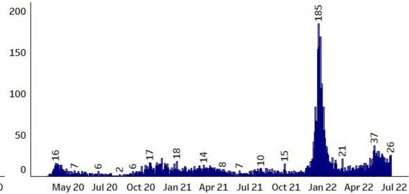
Case Trends (1/1/2020 - 08/02/22)
