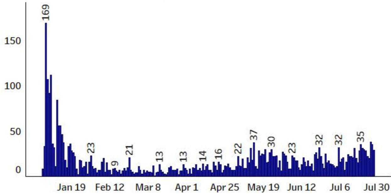
Case Trends (01/01/2021 - 08/02/22)
