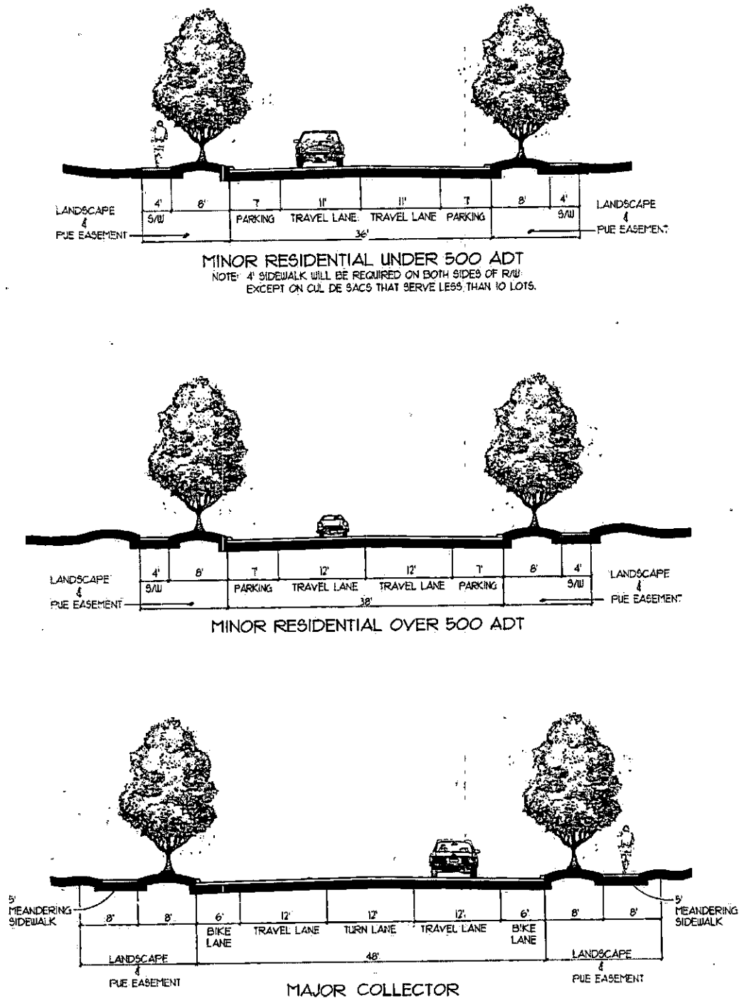
Figure 3.3.2 Minor Road Sections
